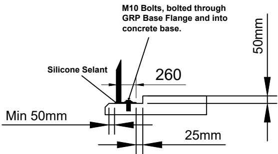
Typical Stepped Concrete Base Detail (Recommended)
