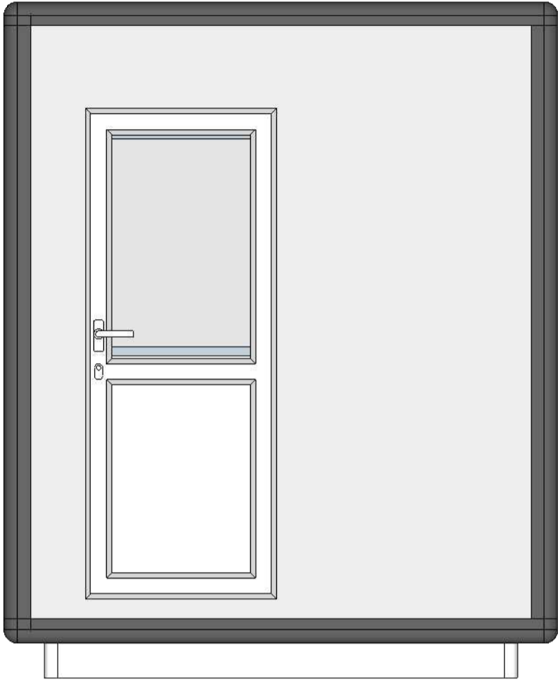
ELEVATION 'A'
